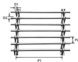
Pre-crimp Wire and Rod Mesh
