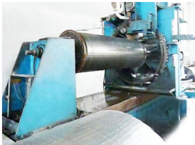
Welding machine
