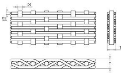
Twilled Dutch Weave
