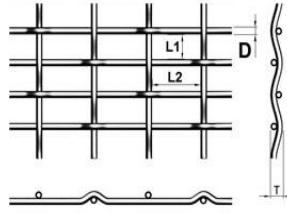
Slot Hole Crimped Weave
