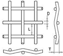
Plain Weave
