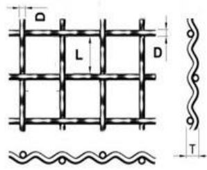
Single Inter Crimp Weave
