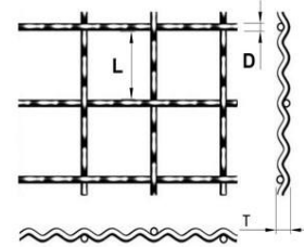
Double Inter Crimp Weave
