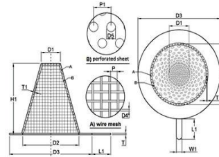
Temporary Basket Strainers
